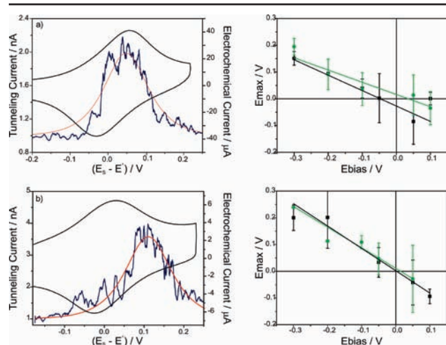
Figure 2. Plots of I_T vs E_S - E^0 (positive-going sweep) recorded in 0.1 M \text{KClO}_4 with E_{\text{bias}} = +0.05 V for (a) Au(111)/PhCOOH/Os and (b) Au(111)/SphCOOH/Os (blue lines, left scale). The red lines correspond to the best fits of I_T to eq 1. The CVs (in 0.1 M \text{NaClO}_4 , 500 \text{mV s}^{-1} ) are also shown (black lines, right scale). Corresponding plots of E_{\text{max}} (the peak position in I_T ) vs E_{\text{bias}} are also shown to the right; ● and ■ symbols denote anodic and cathodic scans, respectively.
